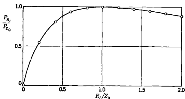
FIG. 7-3.—Effect of load mismatch on power transfer.
